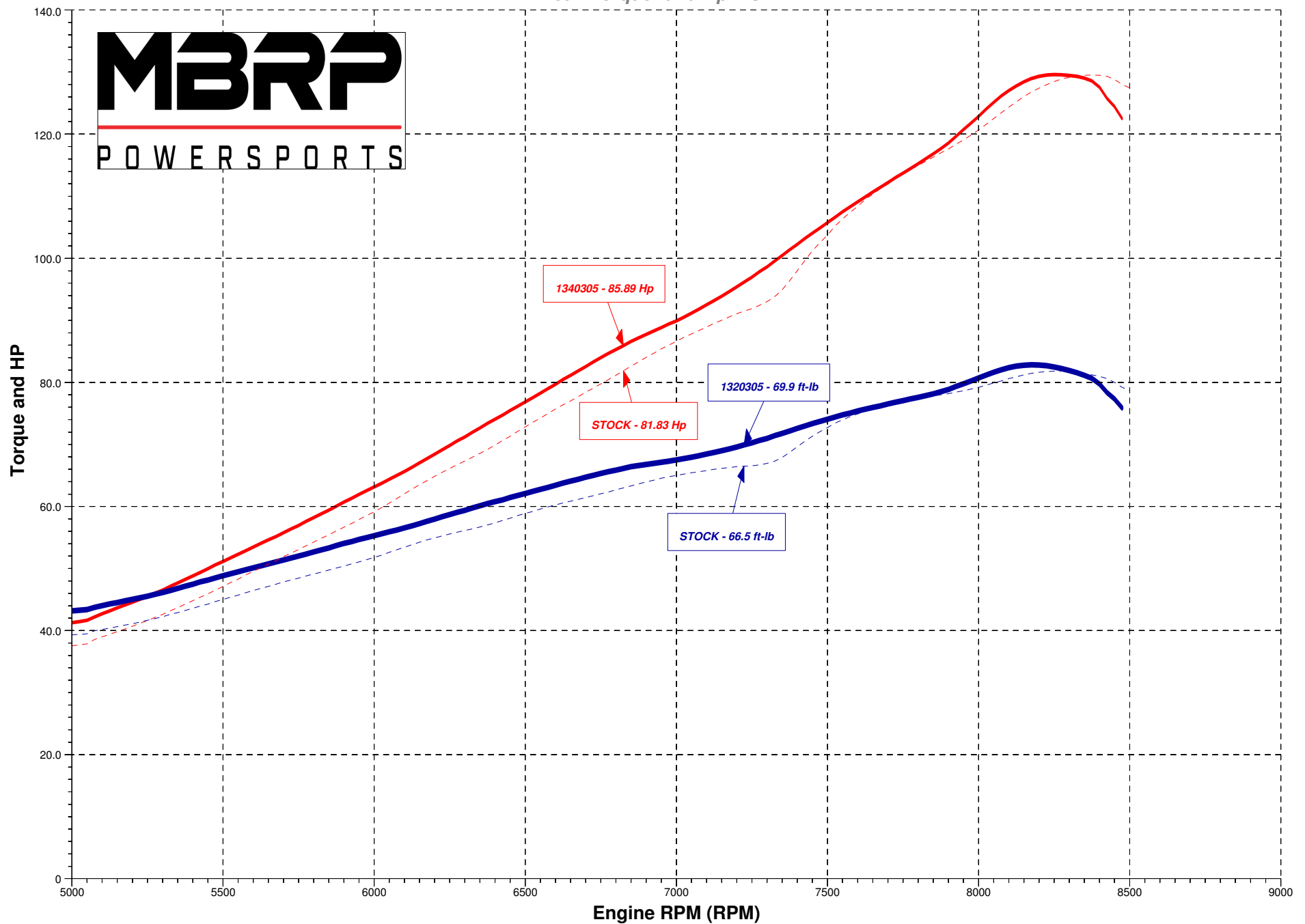
Peak Torque* and Hp* vs. RPM
